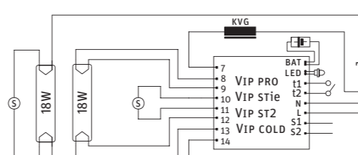
Fig.5. Supply-network and post current-decay mode with two fluorescent lamps 18 W (VIP PRO/VIP STie/VIP ST2/VIP COLD). Emergency mode with one fluorescent lamp.
