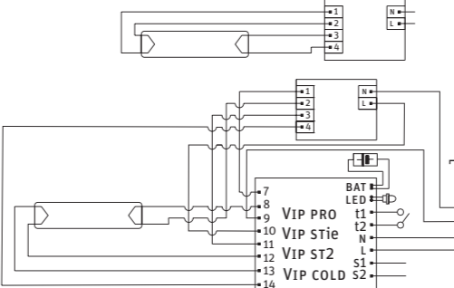
Fig.6. Supply-network and emergency mode with one fluorescent lamp in electronic ballast circuit (VIP PRO/VIP STie/VIP ST2/VIP COLD)
