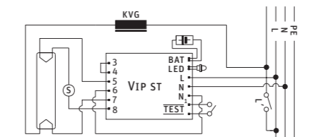
Fig.2. Supply-network and emergency mode with one fluorescent lamp (VIP ST)
