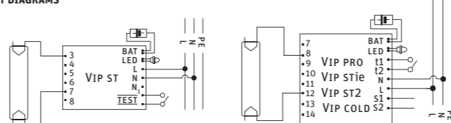
Fig. 1 Emergency mode with one fluorescent lamp (VIP ST, VIP PRO/VIP STie/VIP ST2/VIP COLD)
